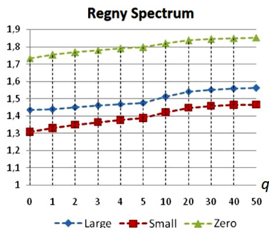
Figure 3. Regny spectra for images of pharmacological solutions of Ag with different concentration
